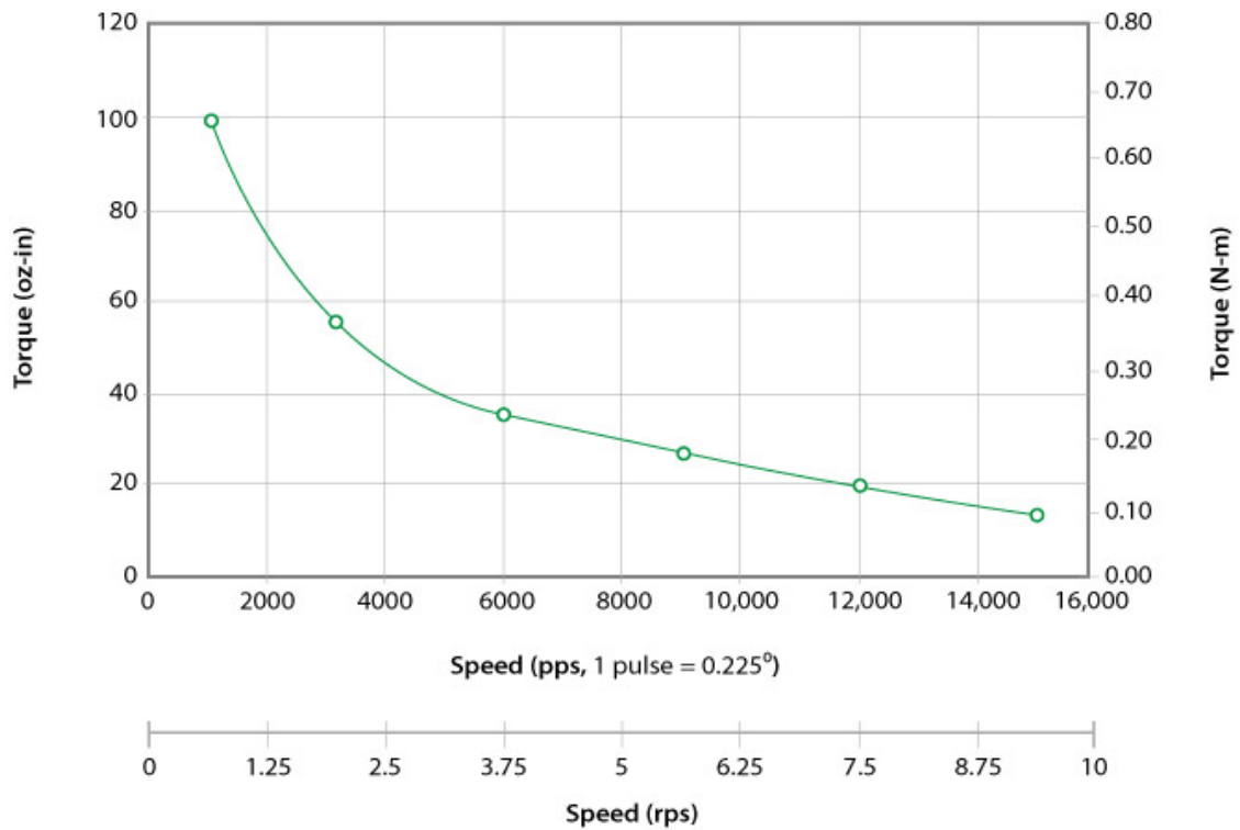
5704M-03 24VDC, 3.0 Amps/Phase, Bipolar, 1/2 Stepping
